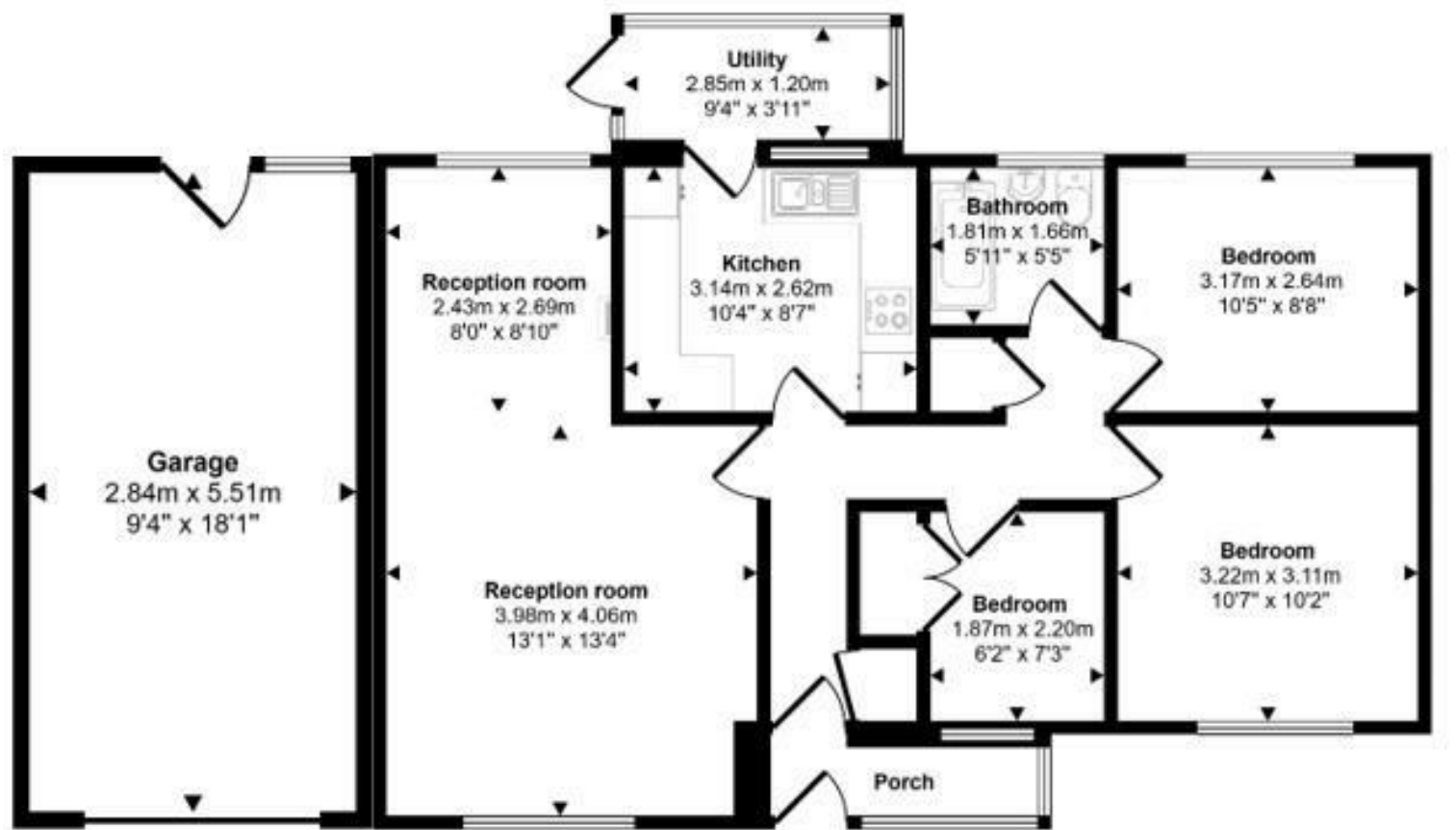
Floorplan Approx 76 sq m / 823 sq ft
